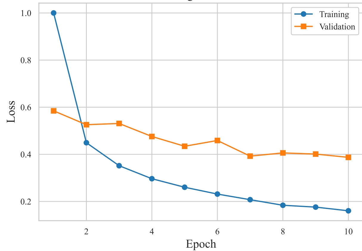
Batch Normalization
