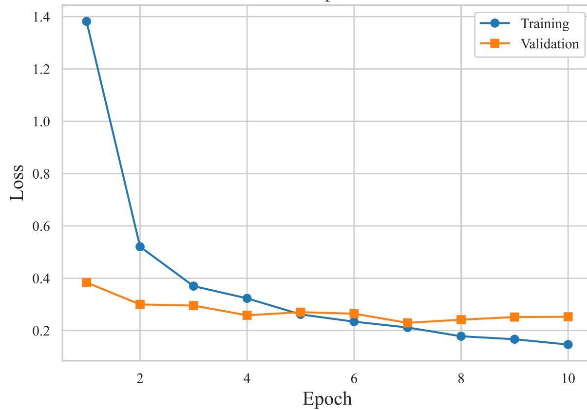
Dropout
